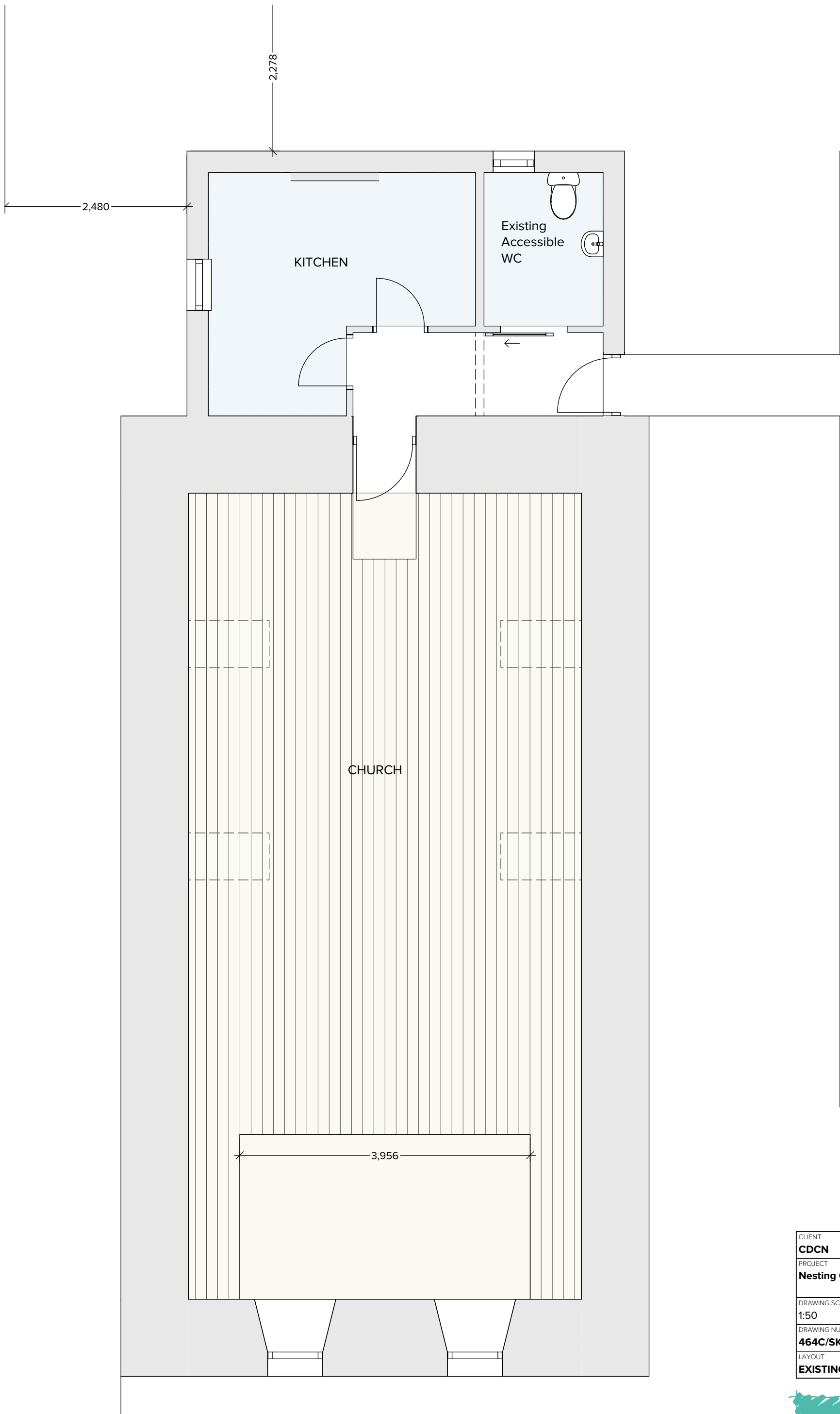
EXISTING FLOOR PLAN 1:50
