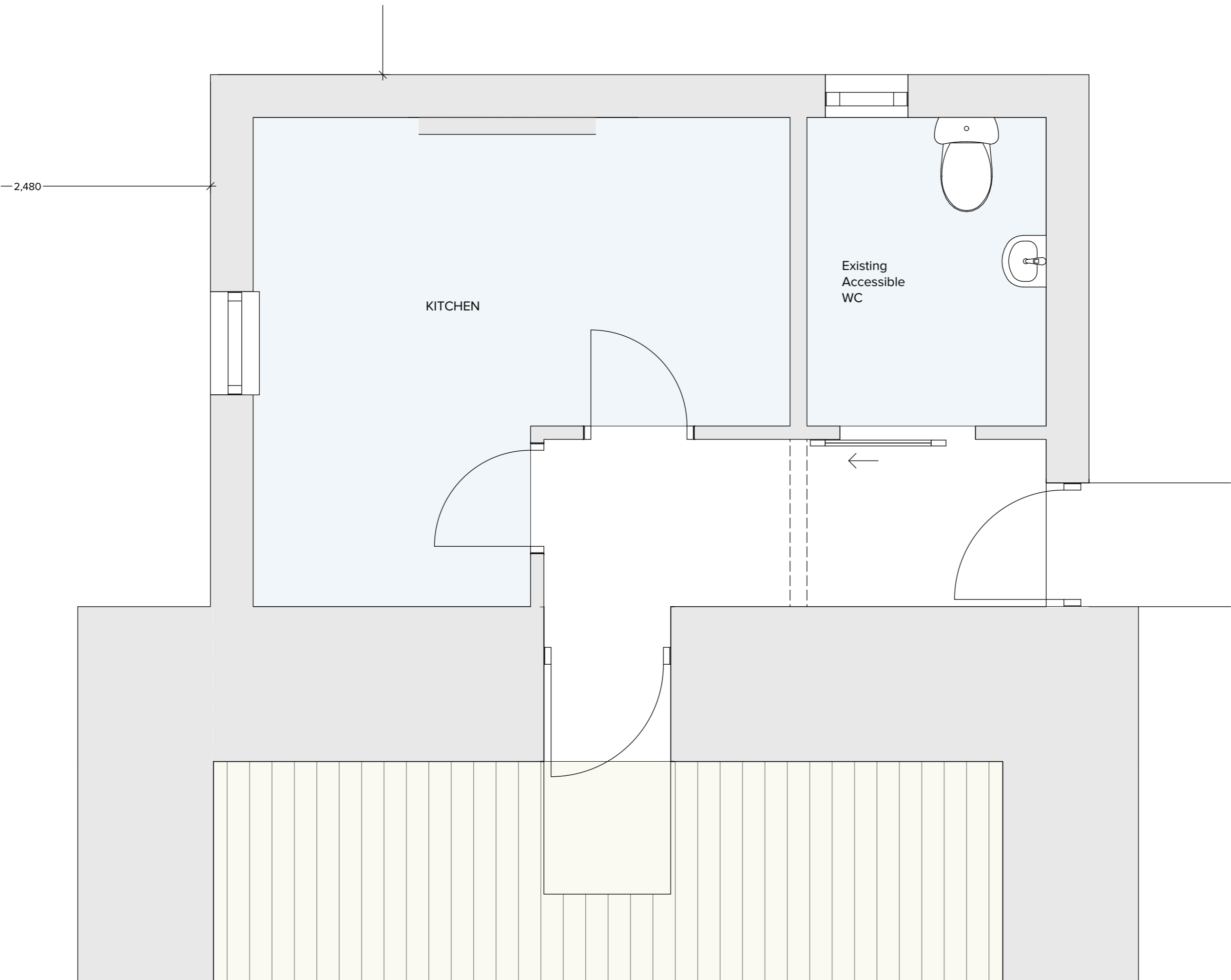
EXISTING VESTRY FLOOR PLAN 1:25
