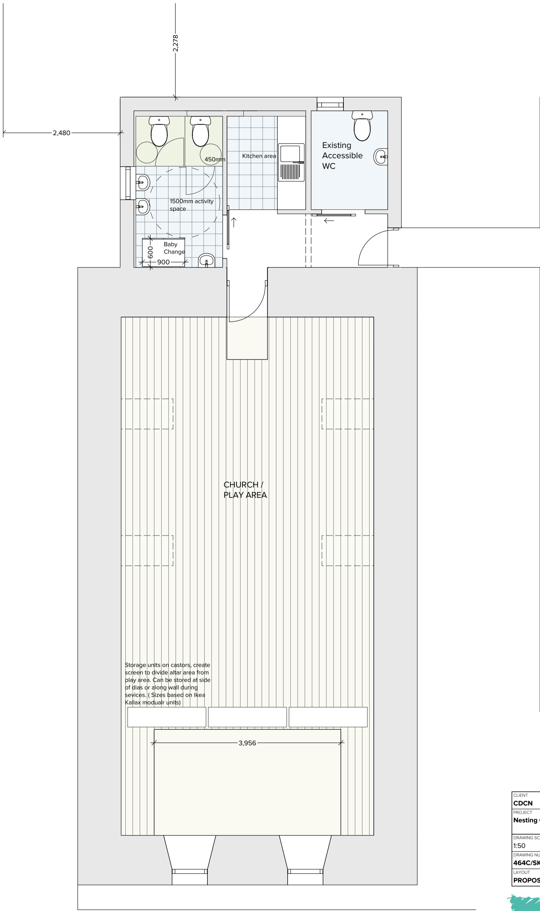
PROPOSED FLOOR PLAN-OPTION 1 1:50
