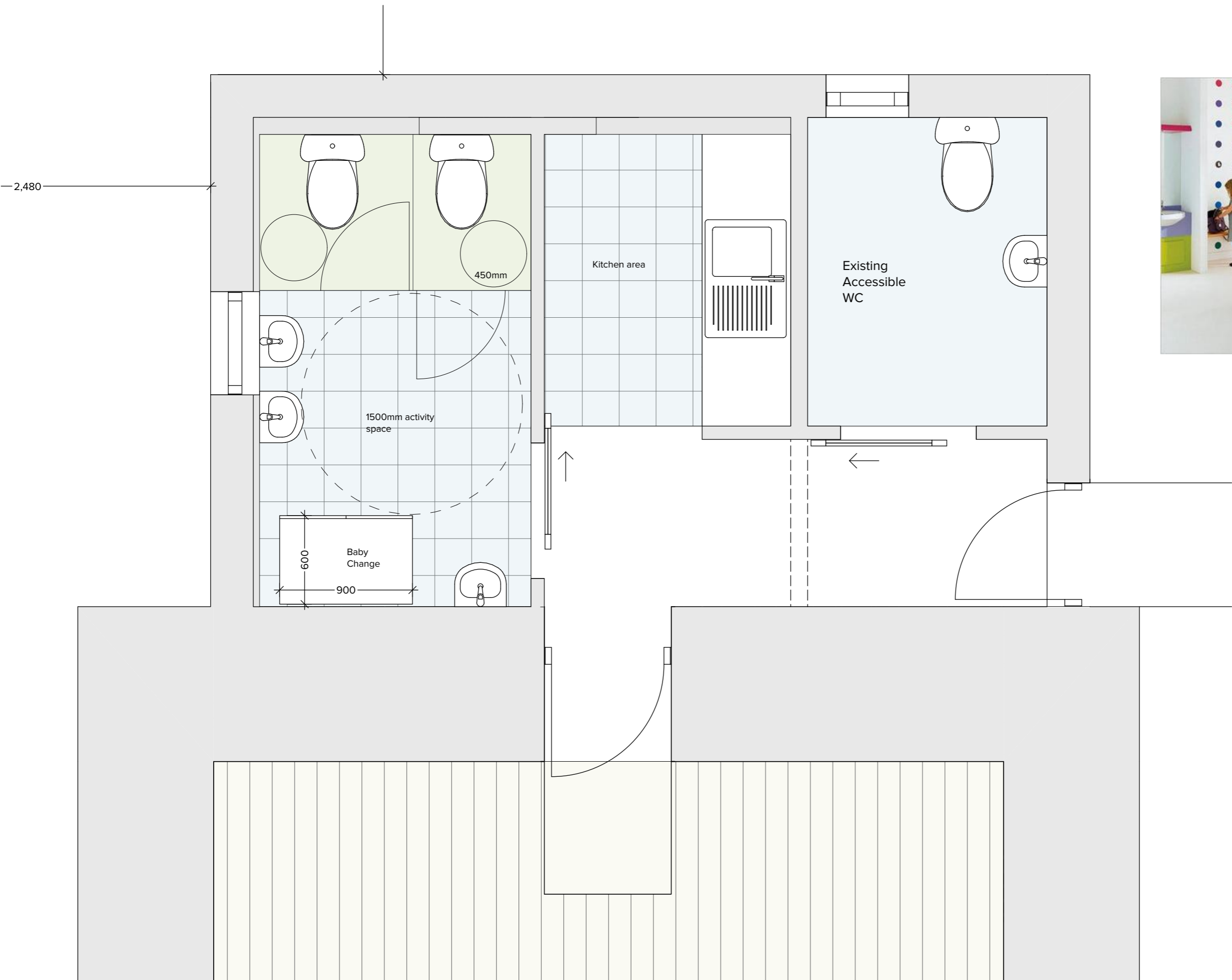
CRECHE FACILITY FLOOR PLAN -OPTION 1 1:25
