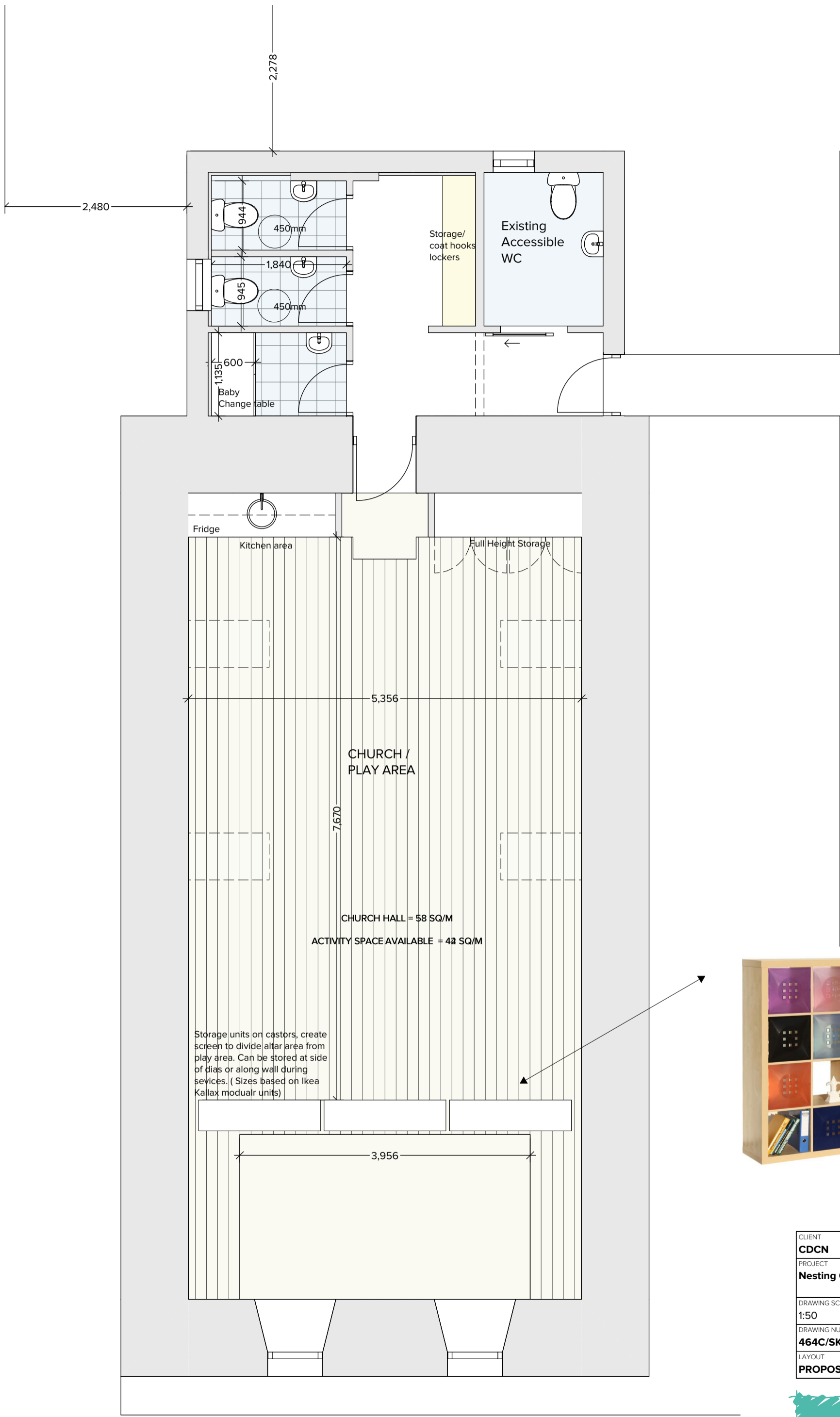
PROPOSED FLOOR PLAN - OPTION 2 1:50
