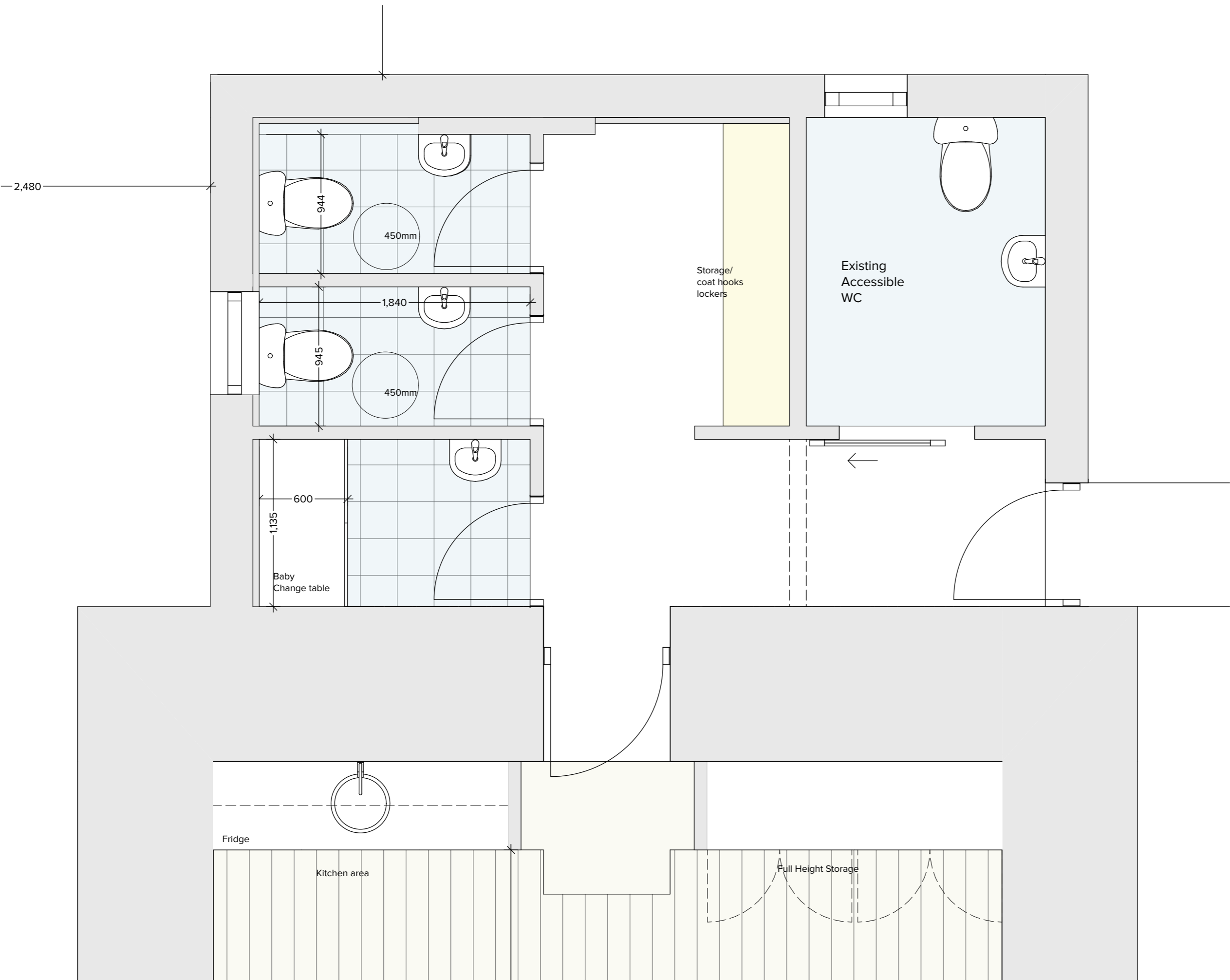
CRECHE FACILITY FLOOR PLAN -OPTION 2 1:25
