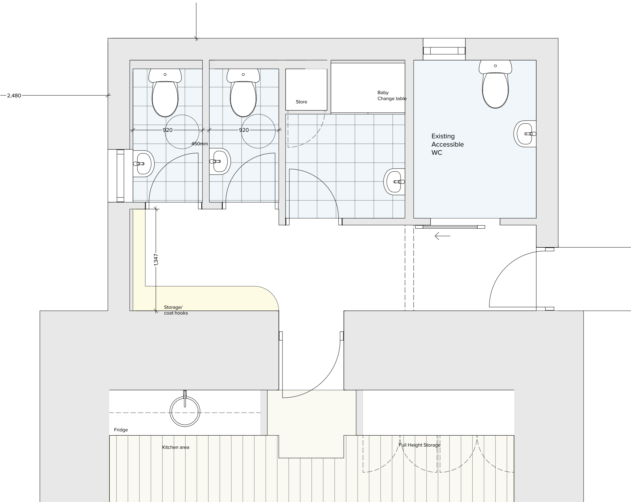
CRECHE FACILITY FLOOR PLAN -OPTION 3 1:25
