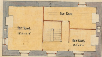
CHAMBER PLAN.
