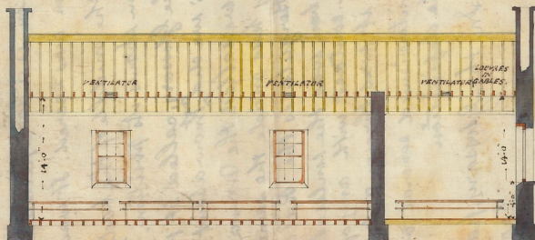
LONGITUDINAL SECTION. (SCHOOL).
