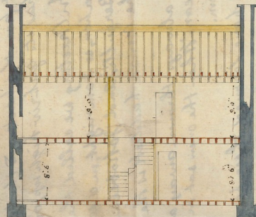
LONGITUDINAL SECTION. (HOUSE)
